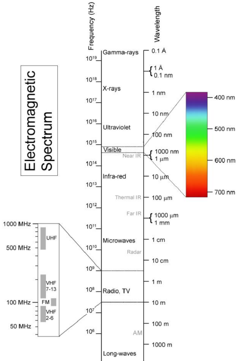
Diagram 1: Electromagnetic Spectrum
